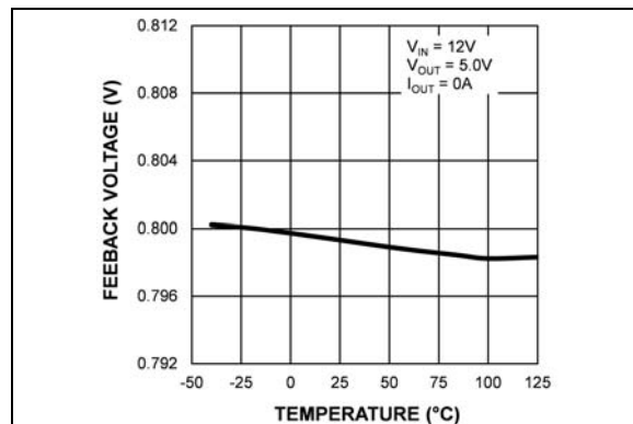
FIGURE 2-23: Feedback Voltage vs. Temperature (MIC28511-2).
