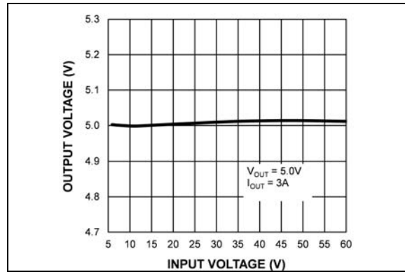
FIGURE 2-22: Output Voltage vs. Input Voltage.
