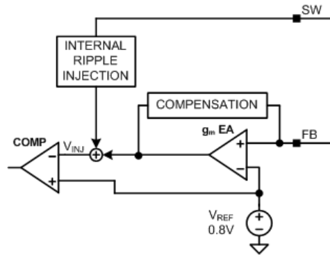
Figure 10. Internal Ripple Injection
