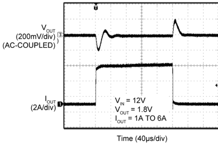
Transient Response
