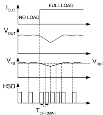
Figure 3. MIC24052 Load Transient Response
