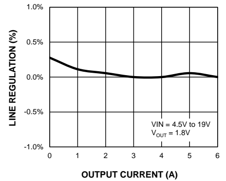
Line Regulation vs. Output Current
