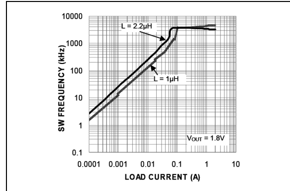
FIGURE 2-16: Switching Frequency vs. Load Current.
