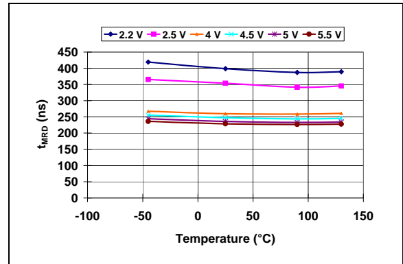
FIGURE 2-38: MR Low to Reset Propagation Delay (MCP1316-2.0).
