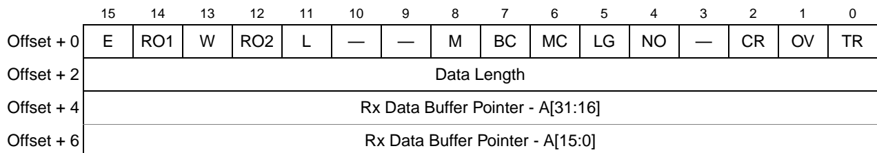
Figure 17-25. Receive Buffer Descriptor (RxBD)
