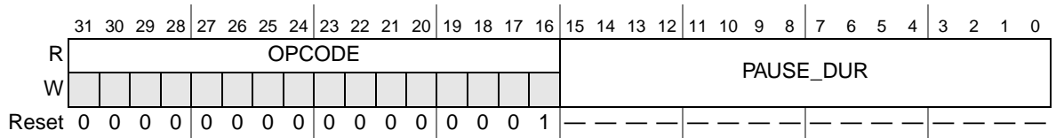
Figure 17-14. Opcode/Pause Duration Register (OPD)
