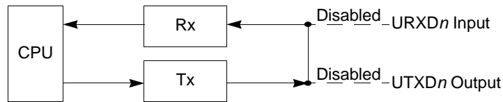
Figure 23-22. Local Loopback
