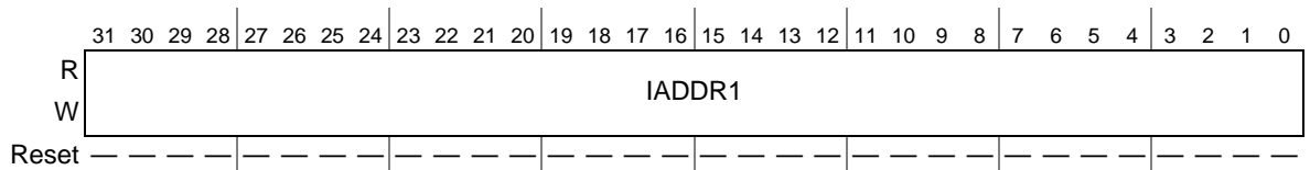
Figure 17-15. Descriptor Individual Upper Address Register (IAUR)
