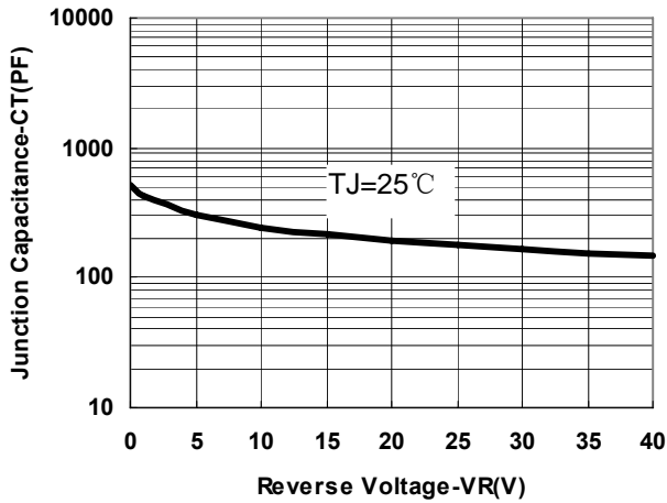
Fig.1-Typical Junction Capacitance
