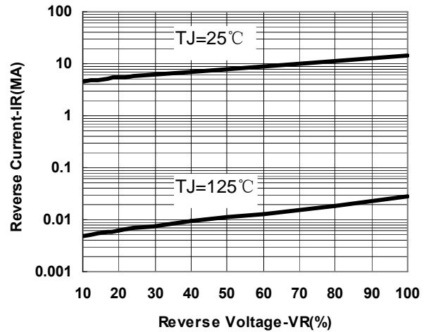
Fig.2-Typical Reverse Characteristics
