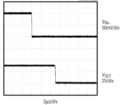
PROPAGATION DELAY ( t_{PD-} ) ( V_{CC} = 3V ) MAX9015 toc36
