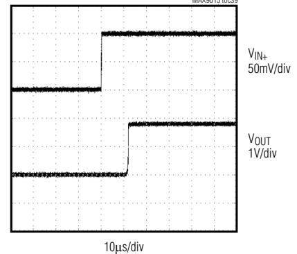
PROPAGATION DELAY ( t_{PD-} ) ( V_{CC} = 1.8V ) MAX9015 toc39
