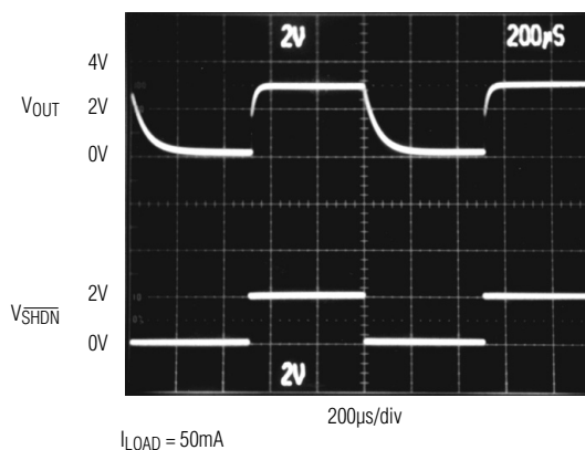
MAX8864 SHUTDOWN
