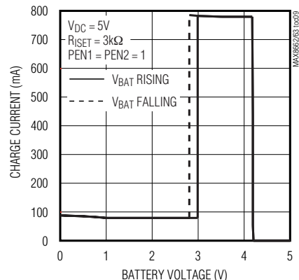
CHARGE CURRENT vs. BATTERY VOLTAGE (AC ADAPTER)
