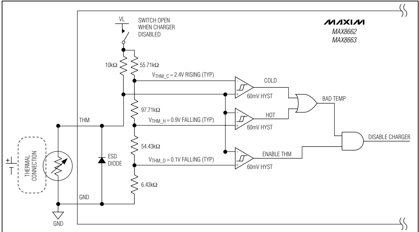
Figure 6. Thermistor Input
