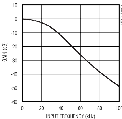
MAX7419/MAX7423 FREQUENCY RESPONSE (BESSEL)
