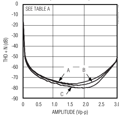
THD + NOISE vs. INPUT SIGNAL AMPLITUDE (BUTTERWORTH)
