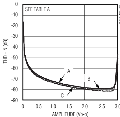
THD + NOISE vs. INPUT SIGNAL AMPLITUDE (ELLIPTIC, r = 1.25 )
