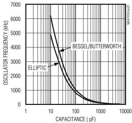
INTERNAL OSCILLATOR FREQUENCY vs. SMALL CAPACITANCE (pF)
