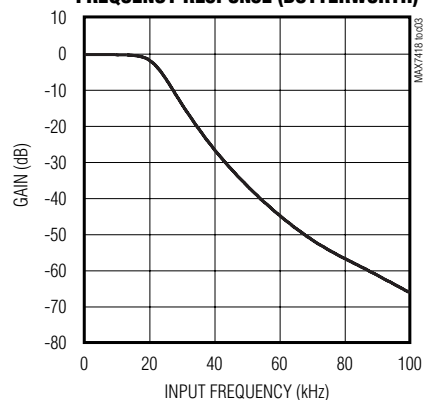
MAX7420/MAX7424 FREQUENCY RESPONSE (BUTTERWORTH)
