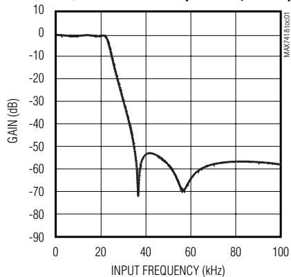
MAX7418/MAX7422 FREQUENCY RESPONSE (ELLIPTIC, r = 1.6 )
