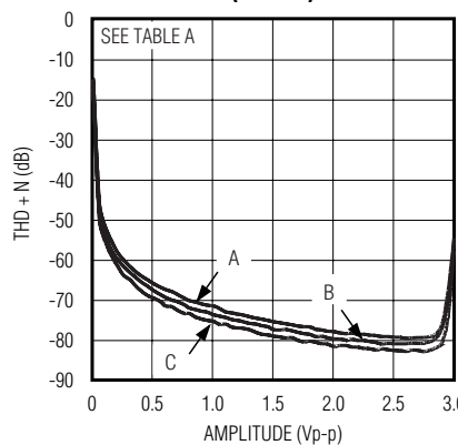
THD + NOISE vs. INPUT SIGNAL AMPLITUDE (BESSEL)
