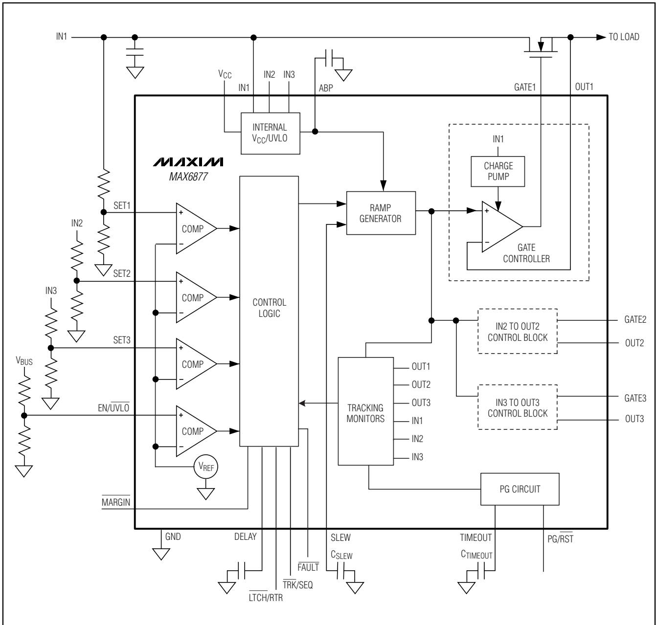
Functional Diagram
