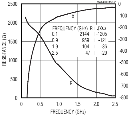
MAX4001 INPUT IMPEDANCE vs. FREQUENCY ( \mu MAX)
