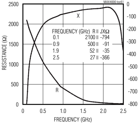
MAX4000 INPUT IMPEDANCE vs. FREQUENCY ( \mu MAX)
