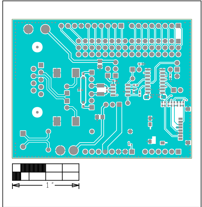
MAX33053E Shield—Top
