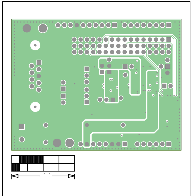
MAX33053E Shield—Internal 3
