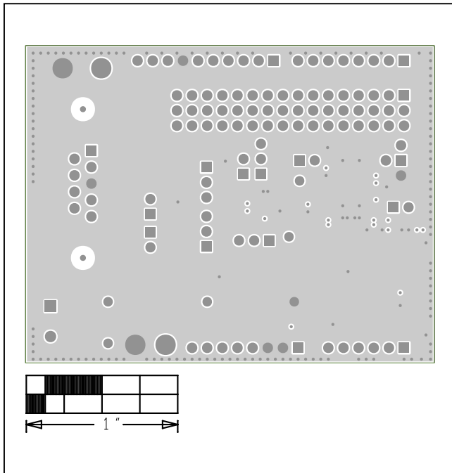
MAX33053E Shield—Internal 2
