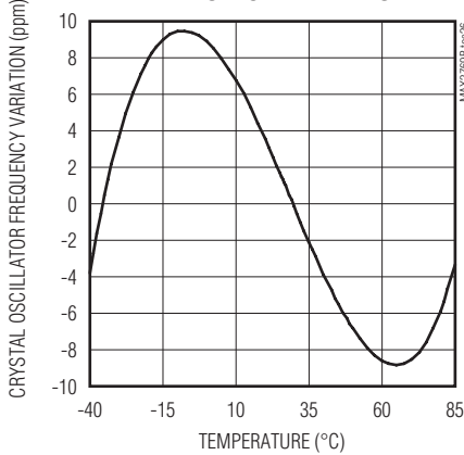
CRYSTAL OSCILLATOR FREQUENCY VARIATION vs. TEMPERATURE
