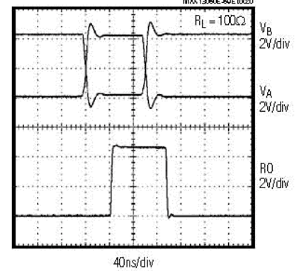
RECEIVER PROPAGATION DELAY (16Mbps)
