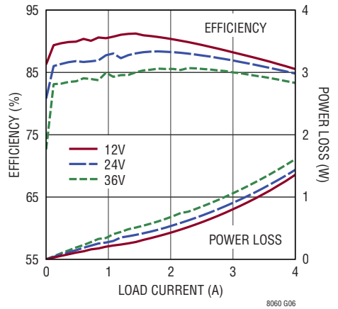
Efficiency and Power Loss V_{OUT} = 2\text{V} , BIAS = 5V, Burst Mode
