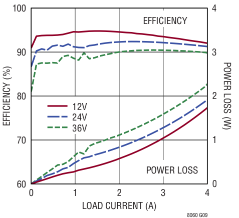
Efficiency and Power Loss V_{OUT} = 5\text{V} , BIAS = 5V, Burst Mode
