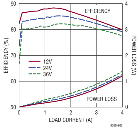
Efficiency and Power Loss V_{OUT} = 1.2\text{V} , BIAS = 5V, Burst Mode
