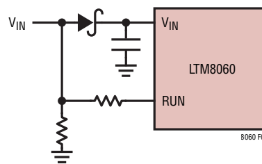
Figure 2. The Input Diode Prevents a Shorted Input from Discharging a Backup Battery Tied to the Output. It Also Protects the Circuit from a Reversed Input. The LTM8060 Runs Only When the Input Is Present.
