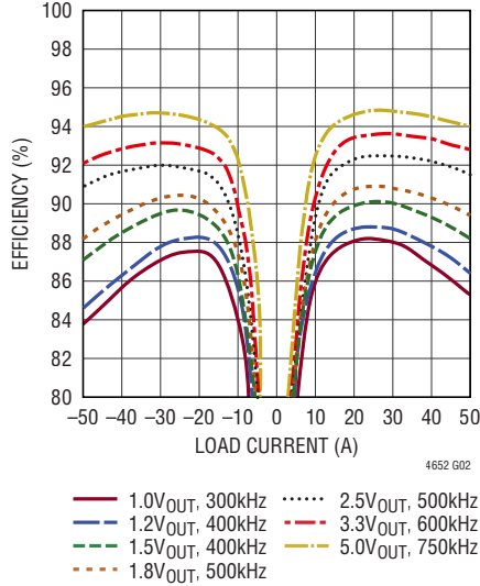
Efficiency vs Output Current, V_{IN} = 12\text{V} , Outputs Paralleled
