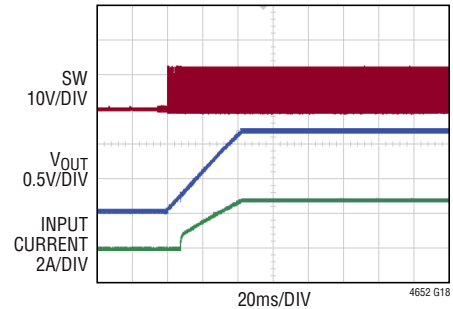
Single Phase Start-Up with 25A Load
