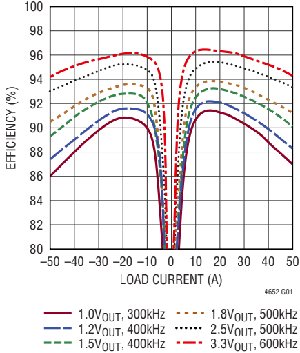
Efficiency vs Output Current, V_{IN} = 5\text{V} , Outputs Paralleled
