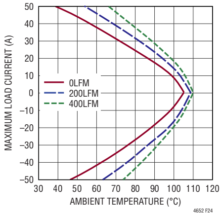
Figure 24. 12V to 1.8V Derating Curve, BGA Heat Sink
