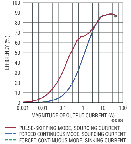
Pulse-Skipping Mode Efficiency V_{IN} = 12\text{V} , V_{OUT} = 1.2\text{V} , f_S = 400\text{kHz} , Outputs Paralleled
