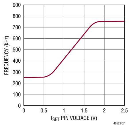
Figure 7. Operating Frequency vs f_{SET} Pin Voltage
