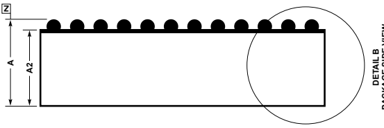
BGA Package 144-Lead (16mm x 16mm x 4.92mm) (Reference DWG # 05-08-7064)
