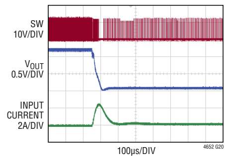
Single Phase Short-Circuit Protection with 25A Load
