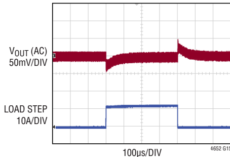
3.3V Dual Phase Single Output Load Transient Response (Bulk Output Capacitor)
