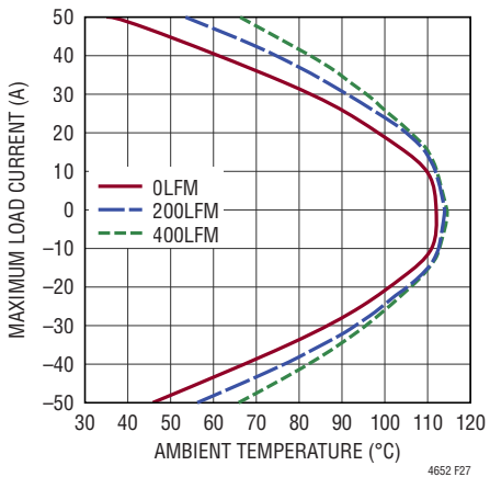
Figure 27. 5V to 3.3V Derating Curve, No Heat Sink
