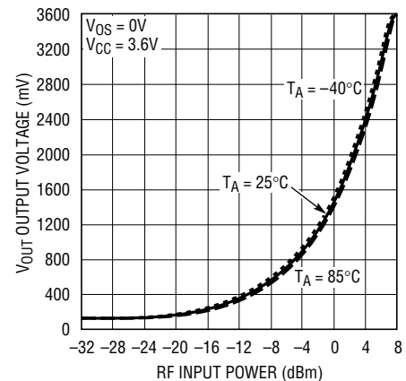
Typical Detector Characteristics, 1000MHz
