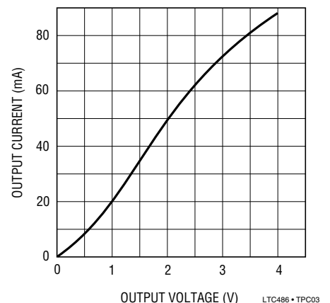
Driver Output Low Voltage vs Output Current T_A = 25^\circ C
