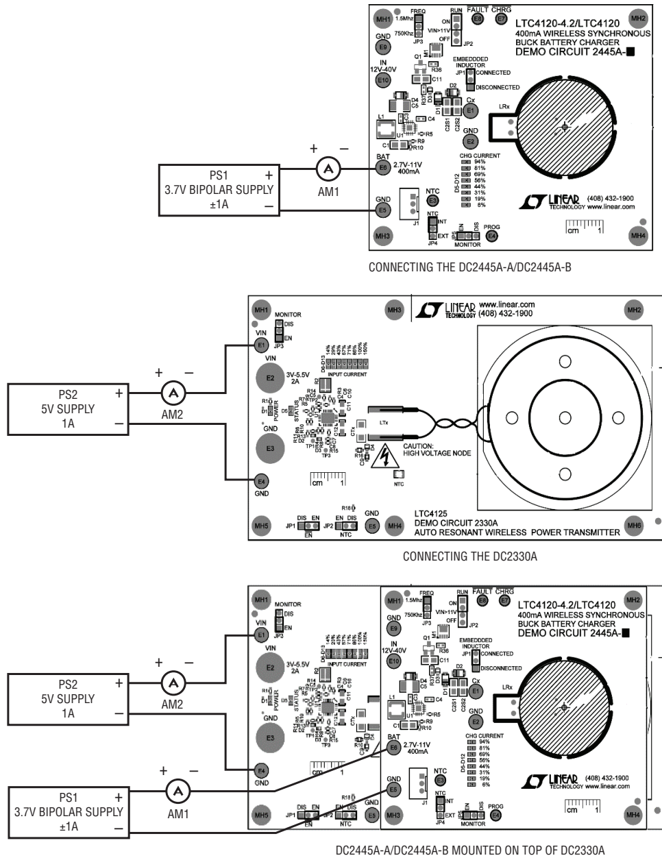
Figure 4. Equipment Setup for DC2386A-A/DC2386A-B Kit
