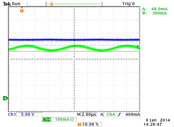
Figure 11. Dk. Blue = LTC4120.IN, Grn. = I(BAT)
