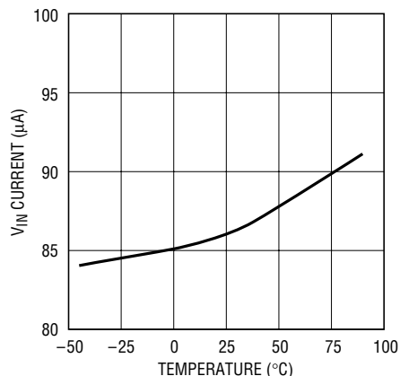
V_{IN} Burst Quiescent Current vs Temperature
