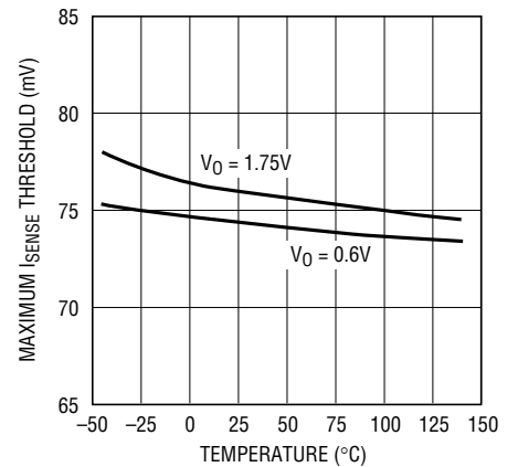
Maximum I_{SENSE} Threshold vs Temperature
