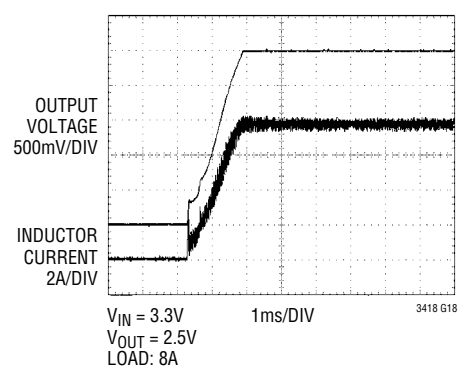
Start-Up Transient
