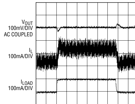
VIN = 3.6V VOUT = 1V ILOAD = 100mA TO 200mA
