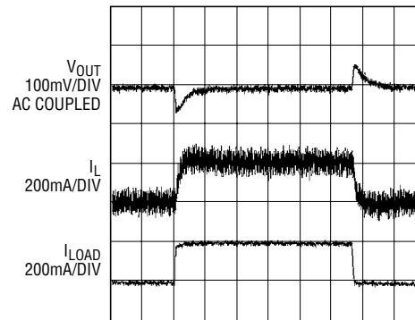
VIN = 3.6V VOUT = 1.2V ILOAD = 100mA TO 300mA
