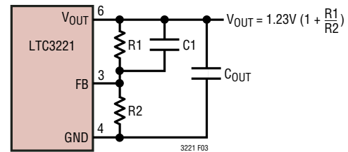
Figure 3. Programming the Adjustable LTC3221
