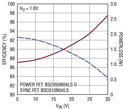
Efficiency and Power Loss vs Input Voltage (1-Phase Using LTC4449)
