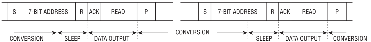
Figure 6. Consecutive Reading at the Same Configuration
