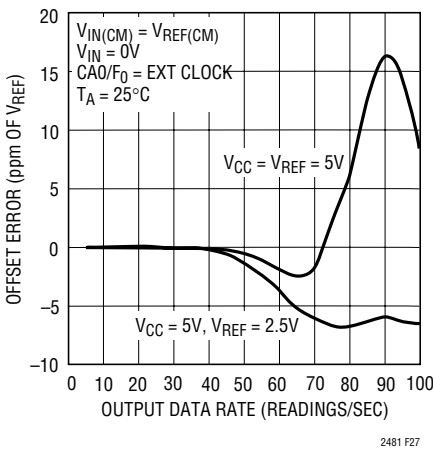
Figure 26. Offset Error vs Output Data Rate and Reference Voltage
