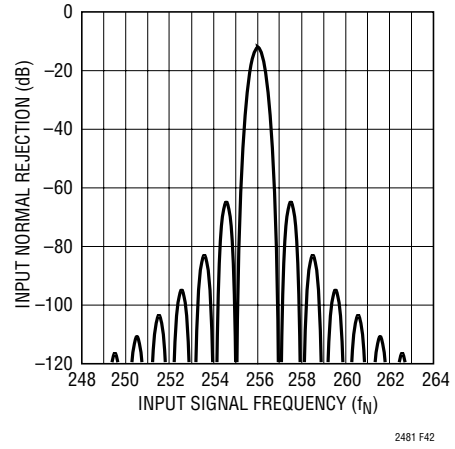
Figure 41. Input Normal Mode Rejection 2x Speed Mode
