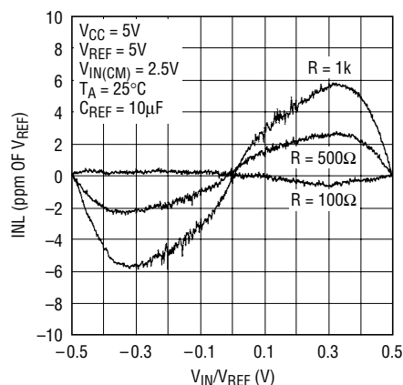
Figure 20. INL vs DIFFERENTIAL Input Voltage and Reference Source Resistance for C REF > 1μF
