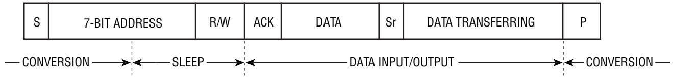
Figure 5. The LTC2481 Conversion Sequence
