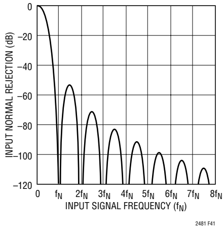
Figure 40. Input Normal Mode Rejection 2x Speed Mode
