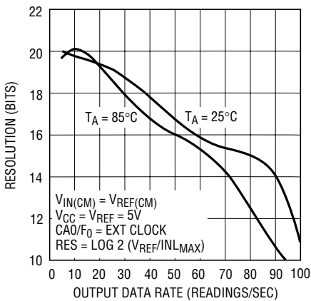
Figure 25. Resolution ( \text{INL}_{\text{MAX}} \leq 1\text{LSB} ) vs Output Data Rate and Temperature
