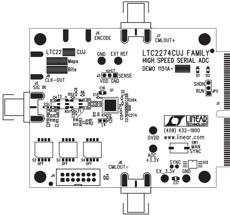
Silkscreen Top
