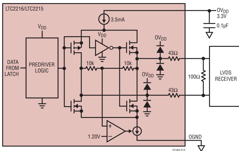
Figure 13. Equivalent Output Buffer in LVDS Mode
