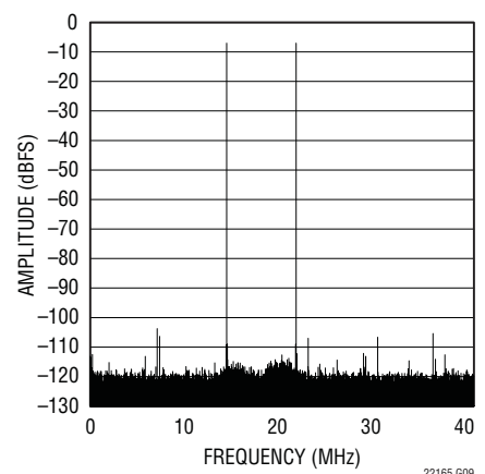
LTC2216 64k Point 2-Tone FFT, f_{IN} = 14.25\text{MHz} and 21.5\text{MHz} , -7dBFS
