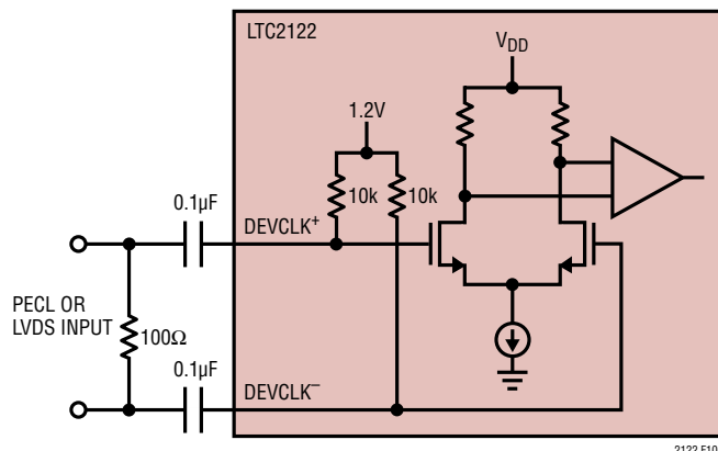
Figure 10. AC Coupled DEVCLK Drive
