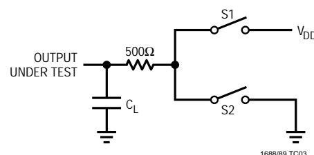
Figure 3. Driver Timing Test Load
