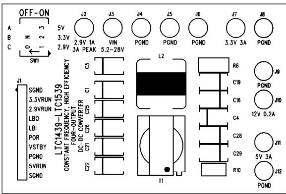
Silkscreen Top
