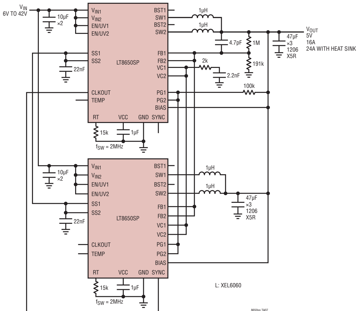
Four Phase, 5V, 24A, 2MHz Step-Down Converter
