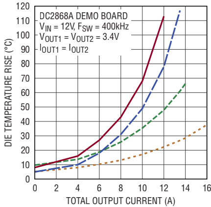
Temperature Rise at 400kHz with Heat Sink and Airflow
