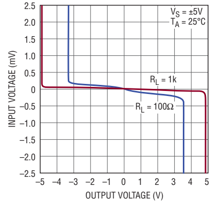
Open-Loop Gain
