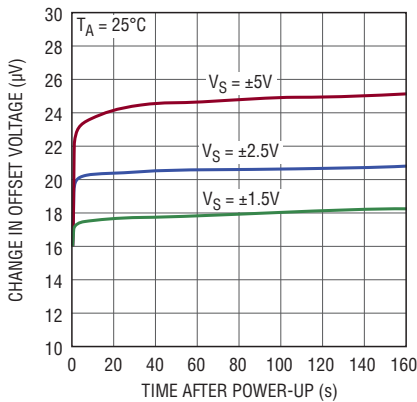
Warm-Up Drift vs Time
