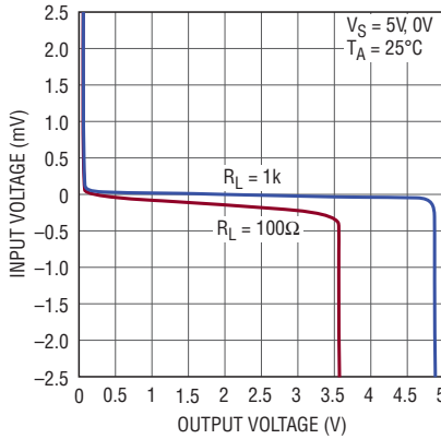
Open-Loop Gain
