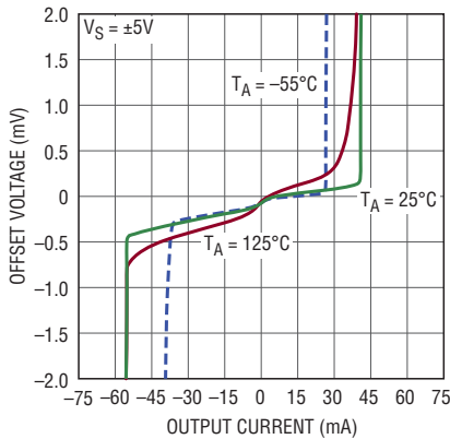
Offset Voltage vs Output Current
