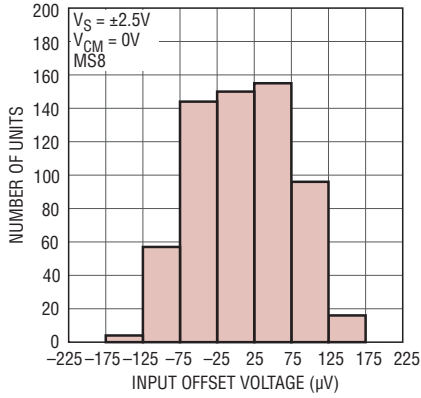
V_{OS} Distribution
