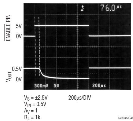
ENABLE Pin Response Time
