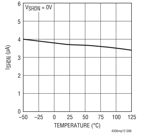
SHDN Current vs Temperature
