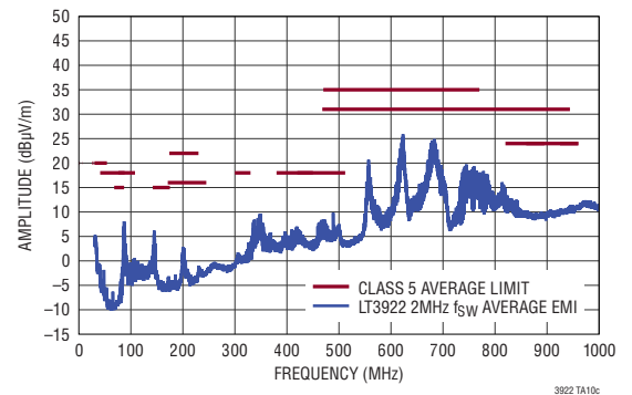
Average Radiated EMI Performance (CISPR25)
