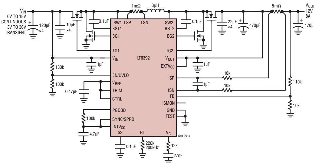
98% Efficient 96W (12V 8A) Buck-Boost Voltage Regulator
