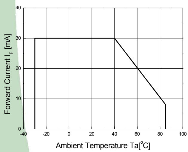
Ambient Temperature vs. Maximum Forward Current
