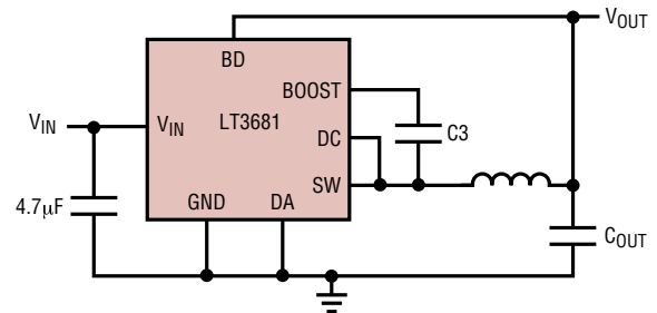
(5a) For V_{OUT} > 2.8V
