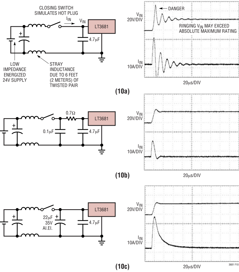
Figure 10. A Well Chosen Input Network Prevents Input Voltage Overshoot and Ensures Reliable Operation when the LT3681 is Connected to a Live Supply
