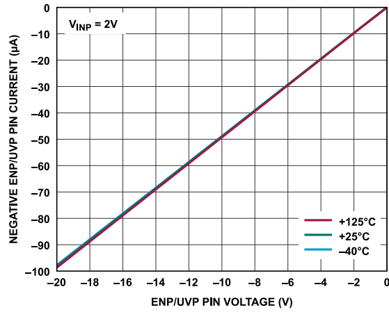
Figure 50. Negative ENP/UVN Pin Current vs. ENP/UVN Pin Voltage
