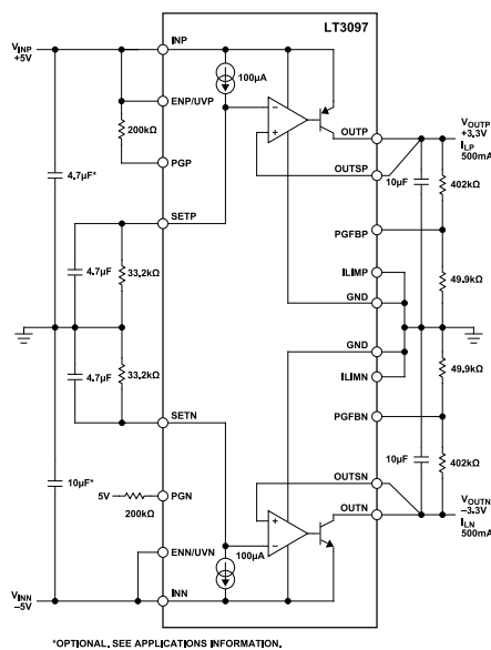
Figure 1. Typical Application
