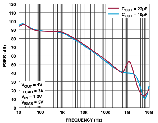
Figure 48. IN Pin PSRR
