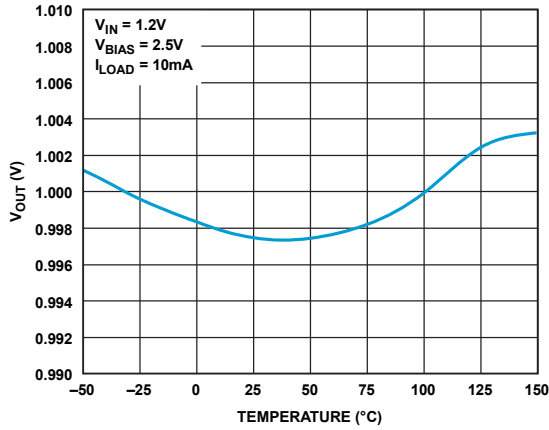
Figure 10. Output Voltage
