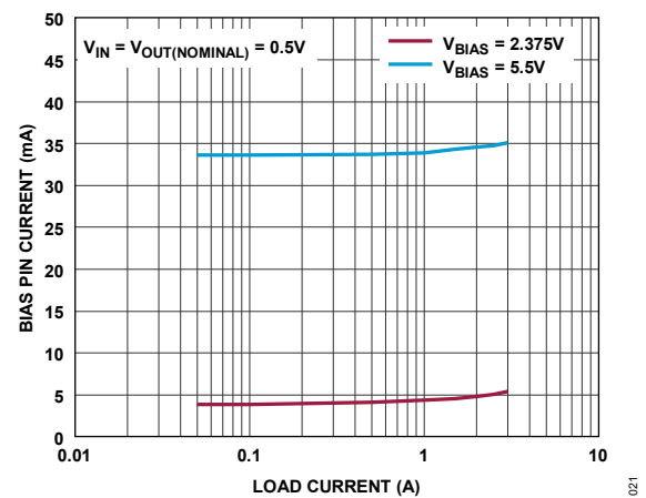
Figure 21. BIAS Pin Current in Dropout
