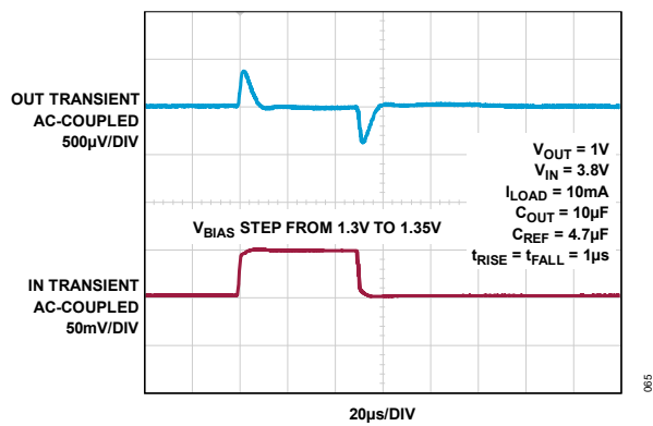
Figure 65. IN Pin Line Transient
