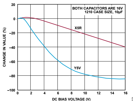
Figure 72. Ceramic Capacitor DC Bias Characteristics
