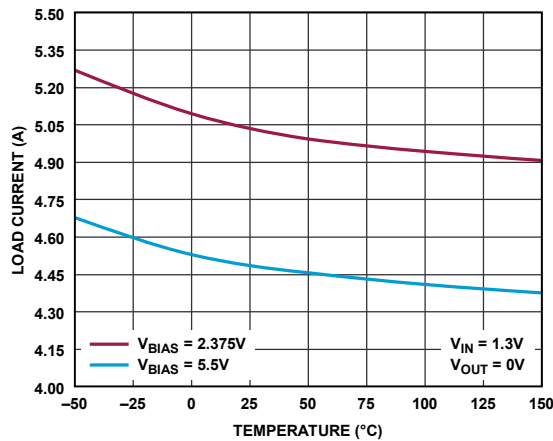
Figure 41. Internal Current Limit
