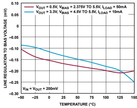
Figure 44. Line Regulation to BIAS
