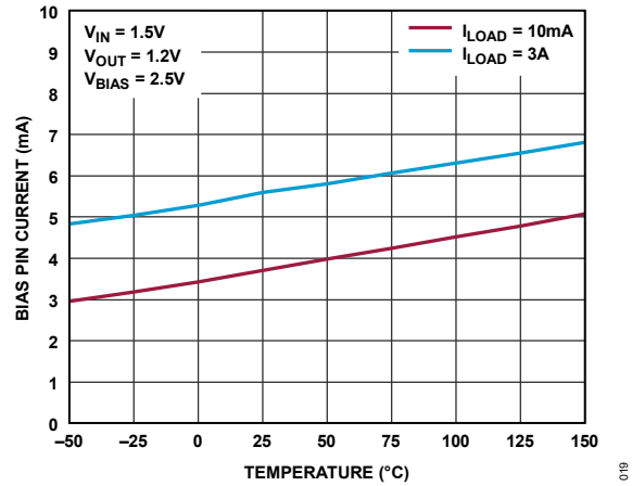
Figure 19. BIAS Pin Current
