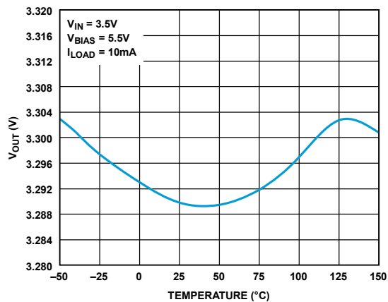
Figure 12. Output Voltage
