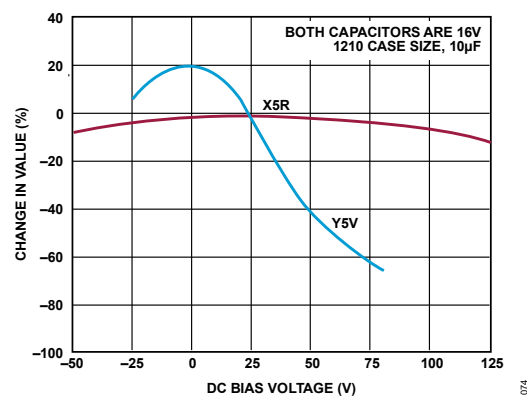
Figure 73. Ceramic Capacitor Temperature Characteristics
