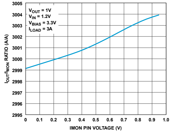
Figure 37. I OUT /I MON Ratio
