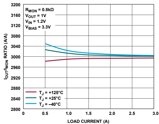
Figure 36. I OUT /I MON Ratio
