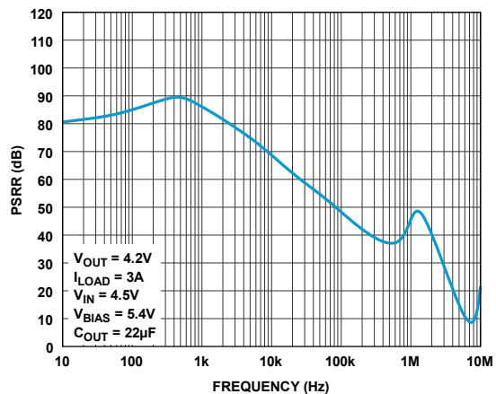
Figure 51. IN Pin PSRR
