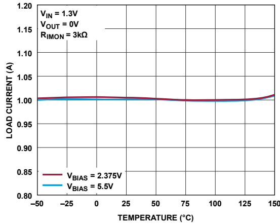
Figure 40. External Current Limit (1A)
