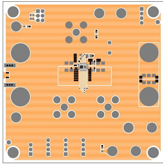
Figure 74. EVAL-LT3073-AZ Evaluation Board
