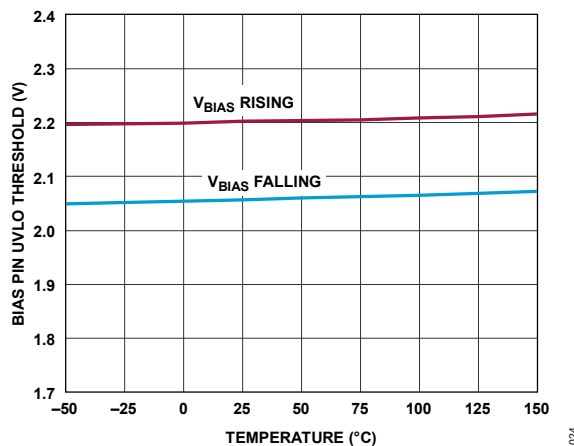
Figure 24. BIAS Pin Undervoltage Lockout Threshold
