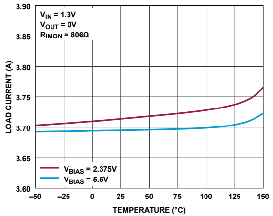
Figure 38. External Current Limit (3.72A)
