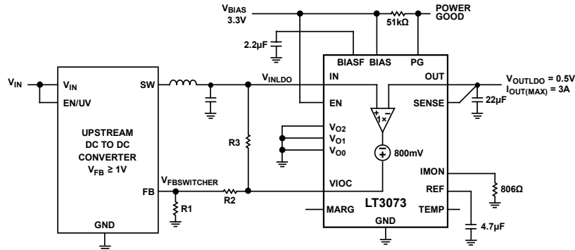
Figure 71. Programming input-to-Output Voltage Differential
