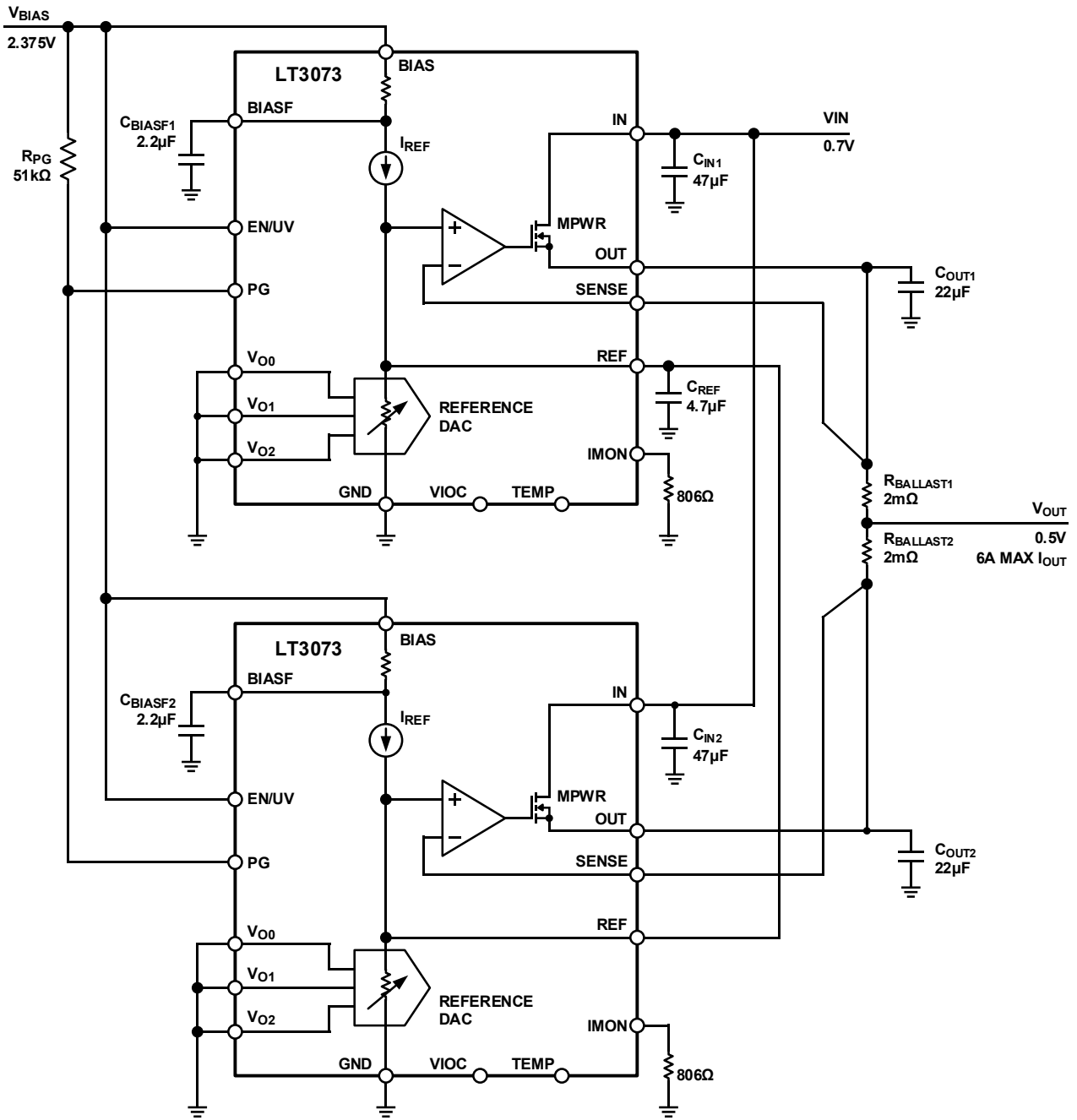
Figure 75. Paralleling Multiple LT3073s for Higher Output Current
