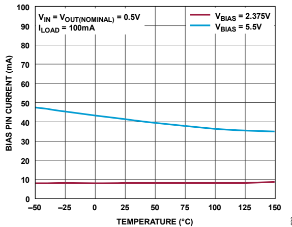
Figure 23. BIAS Pin Current in Dropout
