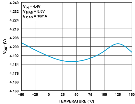
Figure 13. Output Voltage
