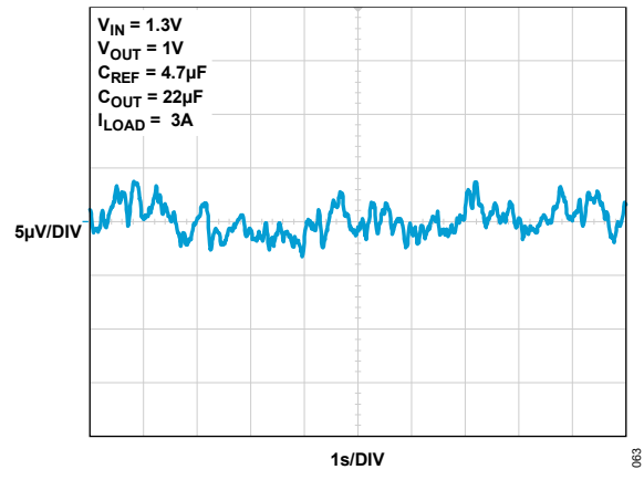
Figure 63. Output Noise (0.1Hz to 10Hz)
