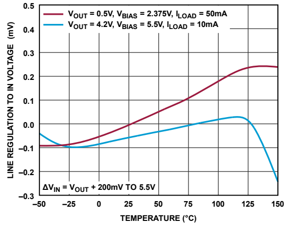
Figure 43. Line Regulation to IN
