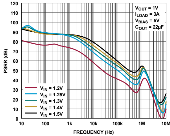
Figure 46. IN Pin PSRR
