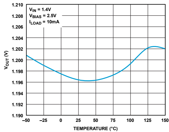
Figure 11. Output Voltage
