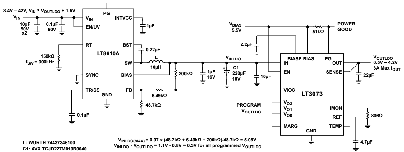
Figure 76. Regulator with VIOC Buck Control
