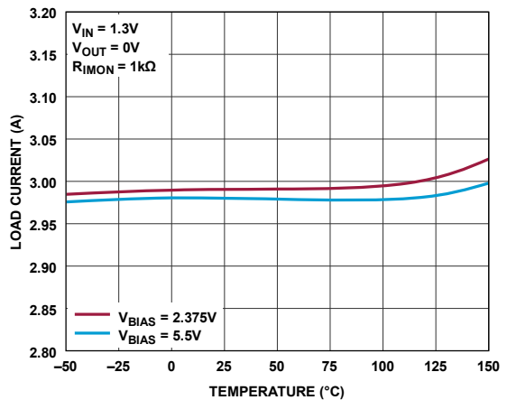
Figure 39. External Current Limit (3A)
