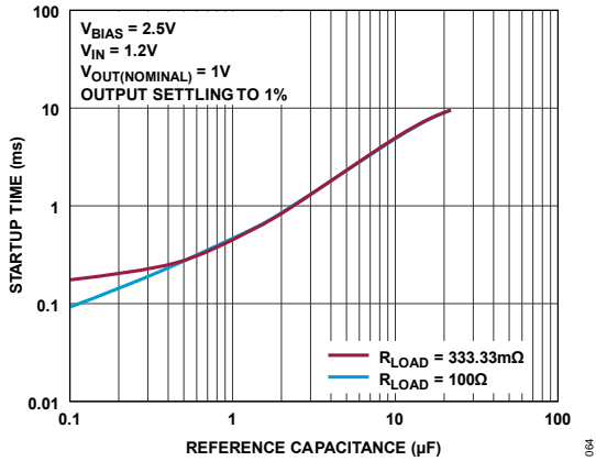
Figure 64. Startup Time
