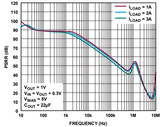
Figure 45. IN Pin PSRR
