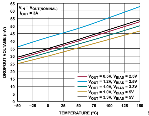
Figure 5. Dropout Voltage (3A)
