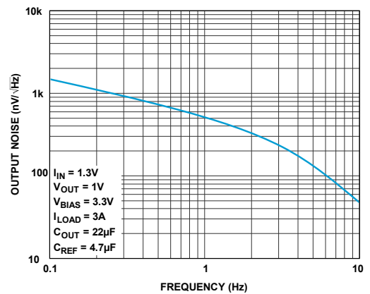
Figure 69. Noise Spectral Density
