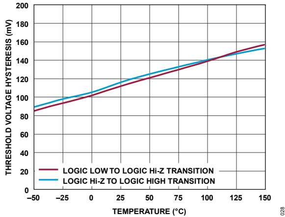
Figure 28. V O0 , V O1 , V O2 and MARG Pin Hysteresis
