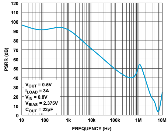
Figure 49. IN Pin PSRR
