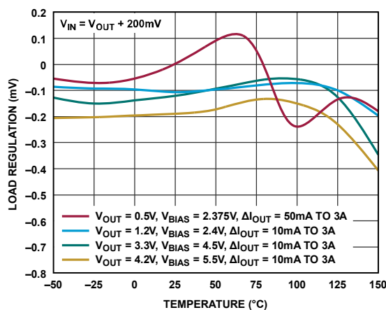
Figure 42. Load Regulation
