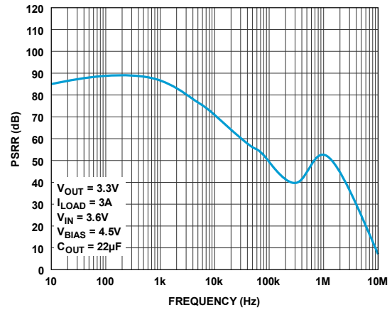
Figure 50. IN Pin PSRR
