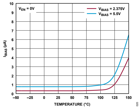
Figure 20. BIAS Pin Current in Nap Mode
