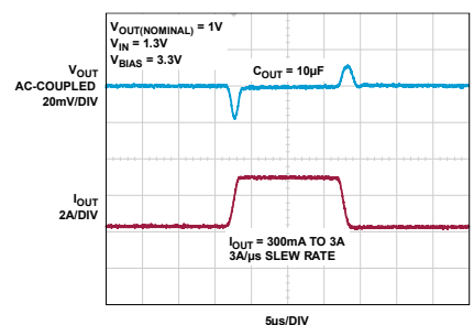
Figure 2. Transient Response
