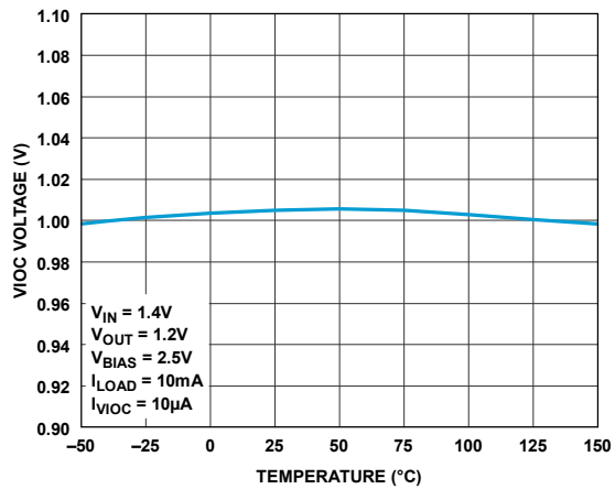
Figure 35. VIOC Pin Voltage
