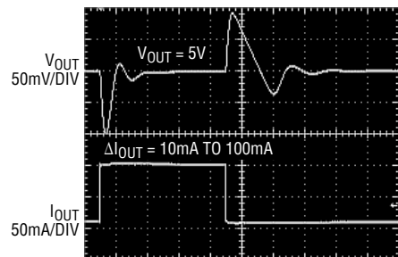
LT3060-5 Transient Response, C_{FF} = 0
