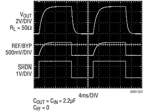
SHDN Transient Response C_{REF/BYP} = 10nF
