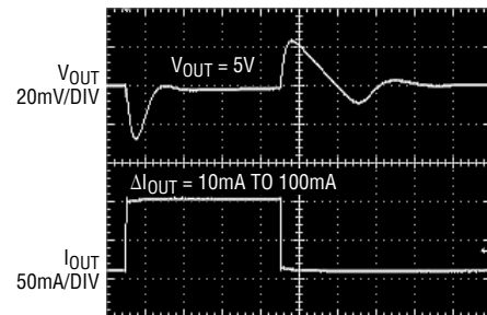
LT3060-5 Transient Response, C_{FF} = 10\text{nF}
