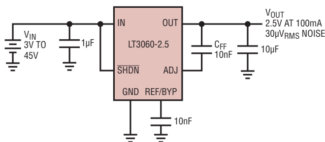
2.5V Low Noise Regulator
