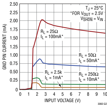
LT3060-2.5 GND Pin Current
