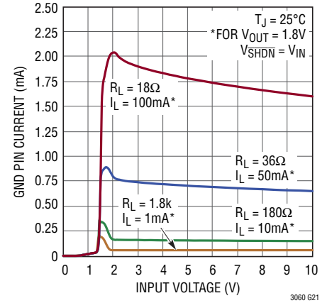
LT3060-1.8 GND Pin Current
