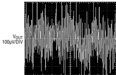
LT3060-5 10Hz to 100kHz Output Noise, C_{REF/BYP} = 10\text{nF} , C_{FF} = 0
