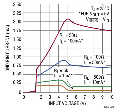
LT3060-5 GND Pin Current
