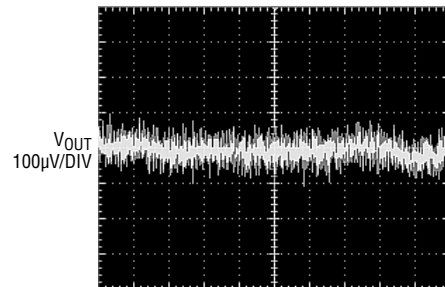
LT3060-5 10Hz to 100kHz Output Noise, C_{REF/BYP} = 10\text{nF} , C_{FF} = 10\text{nF}
