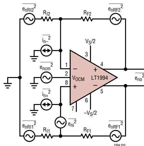
Figure 5. Noise Analysis
