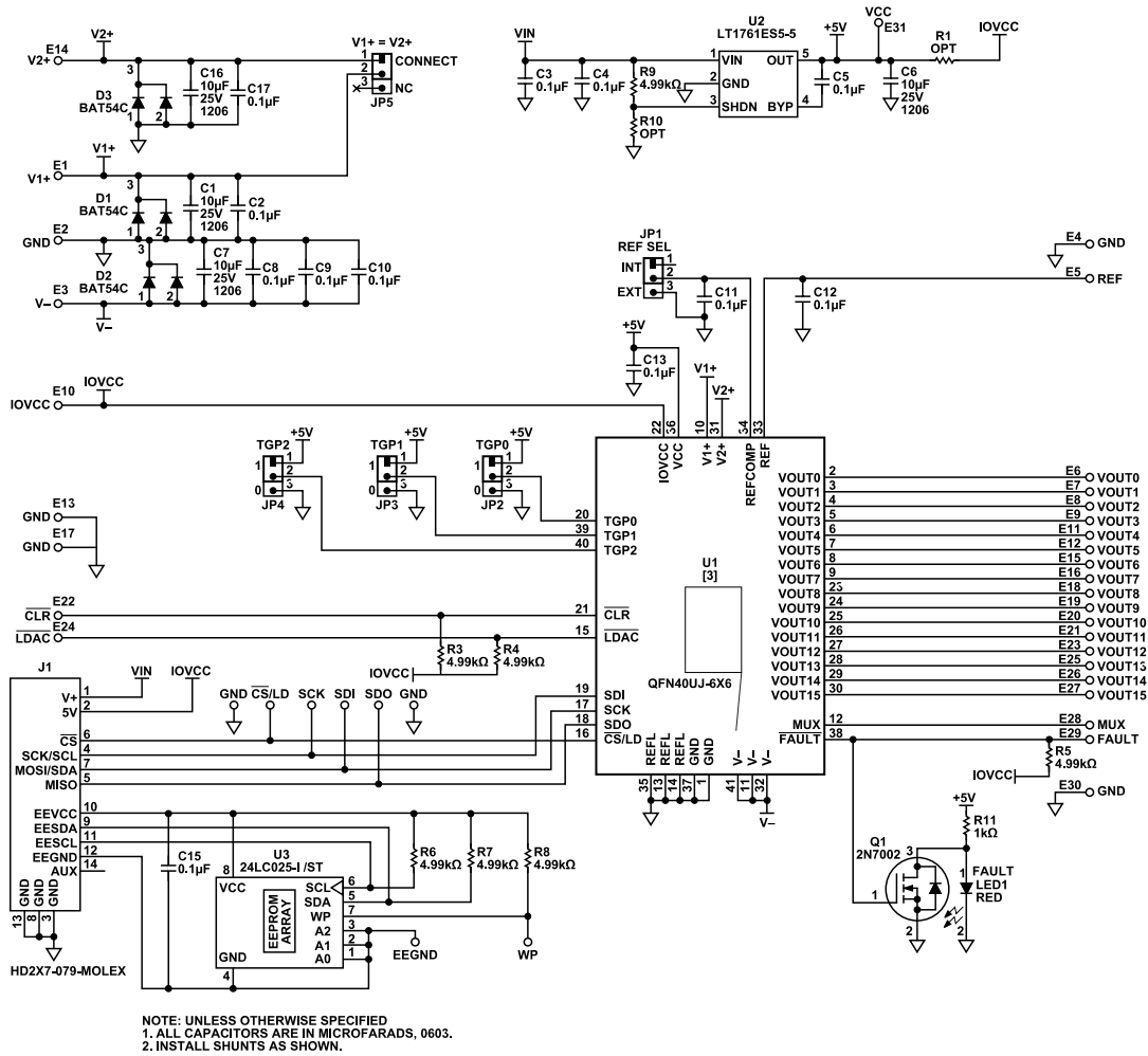
Figure 9. DC2873A-B Schematic
