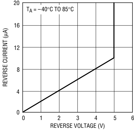
Reverse Characteristics
