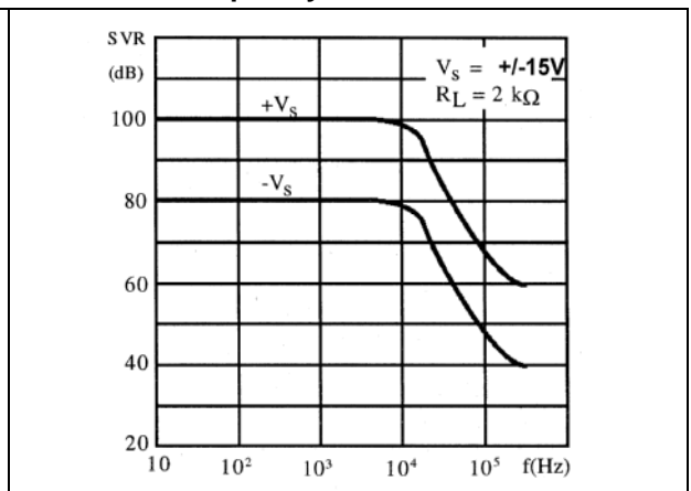
Figure 7. Supply voltage rejection versus frequency
