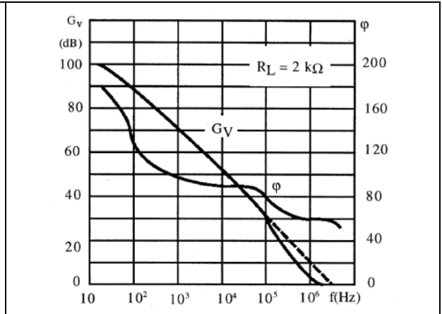
Figure 5. Open loop frequency and phase response
