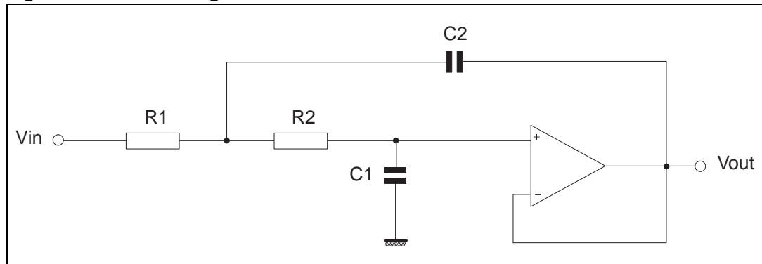
Figure 13. Filter configuration
