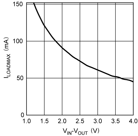
Maximum Load Current vs V_{IN} - V_{OUT} , T_A = 85^\circ\text{C} , V_{OUT} = 1.5\text{V} , SOT23-5 Package
