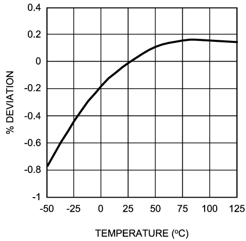
V_{ADJ} vs Temperature
