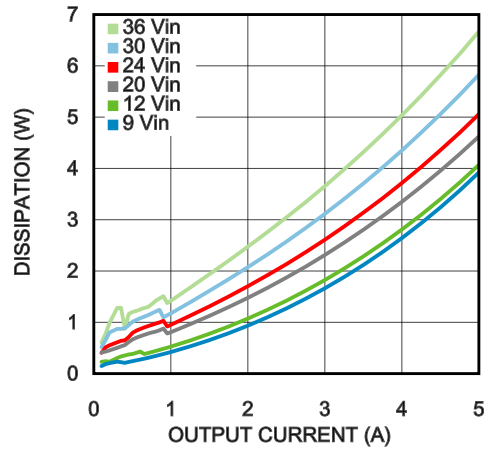
Dissipation 5.0V output @ 25°C ambient
